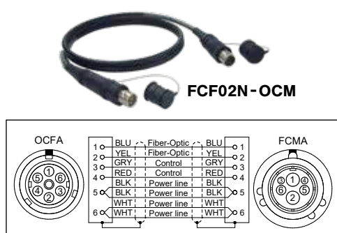
Wiring Diagram for Conversion
