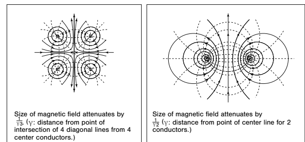
Four-conductor cable
