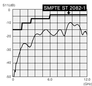
Return Loss for MCVJKA-STW
