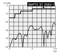
Return loss for BCJ-JK
