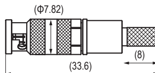
Drawing for HBCP-D25HD
