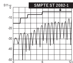
Return loss for HBCP-D25HD
